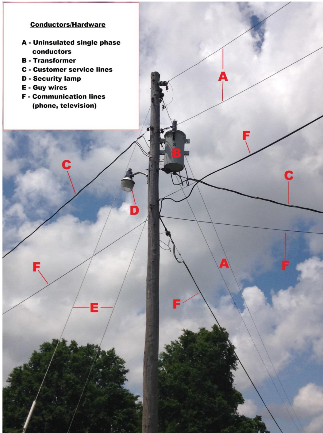
SINGLE PHASE CONSTRUCTION
